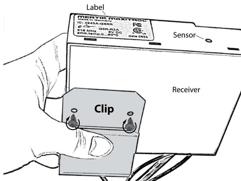
Fixing clip to receiver box
