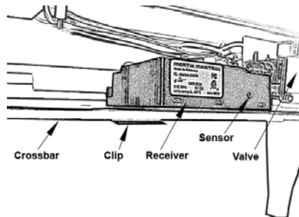
Receiver clipped to crossbar in final position
