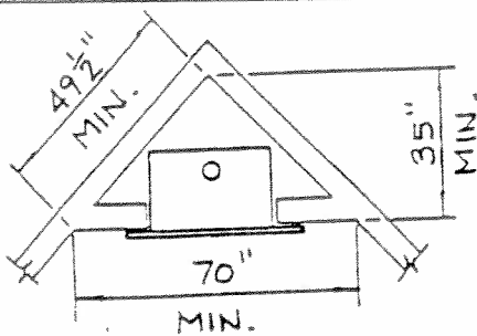
CORNER FRAMING
