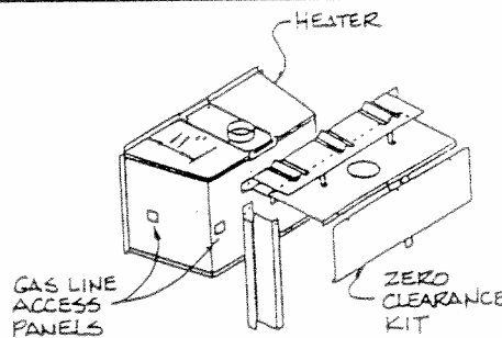
BACK VIEW - ZERO CLEARANCE KIT
