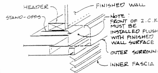
DETAIL - TOP OF FRAMED OPENING
