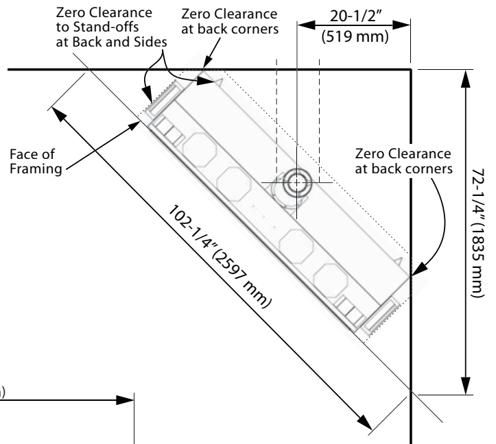
Corner Dimensions
