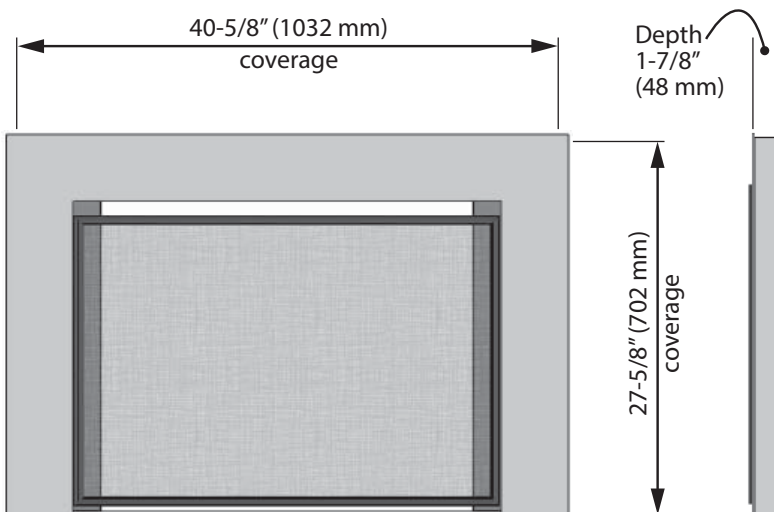
Overall trim slightly larger
